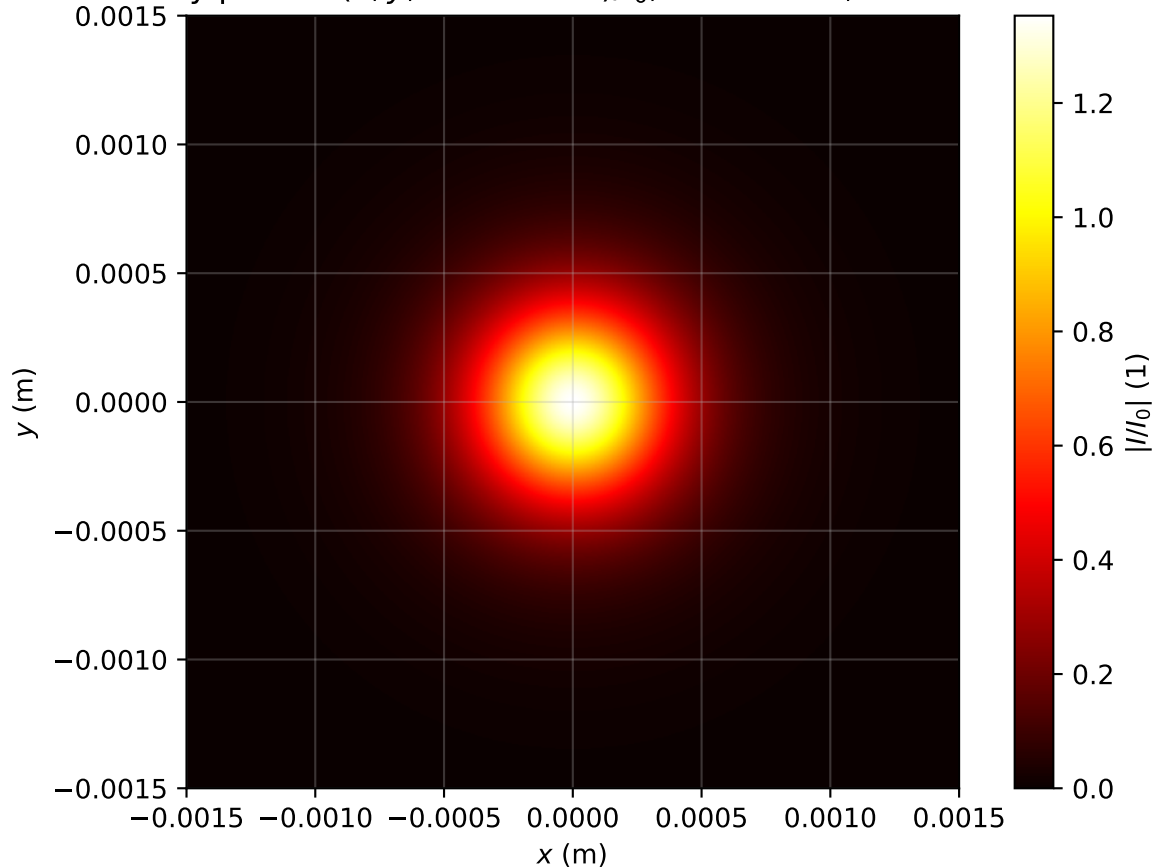
Intensity profile I(x, y, z = 1.672m)/I_0 , P_{in}=0.8P_{cr} , artificial time
